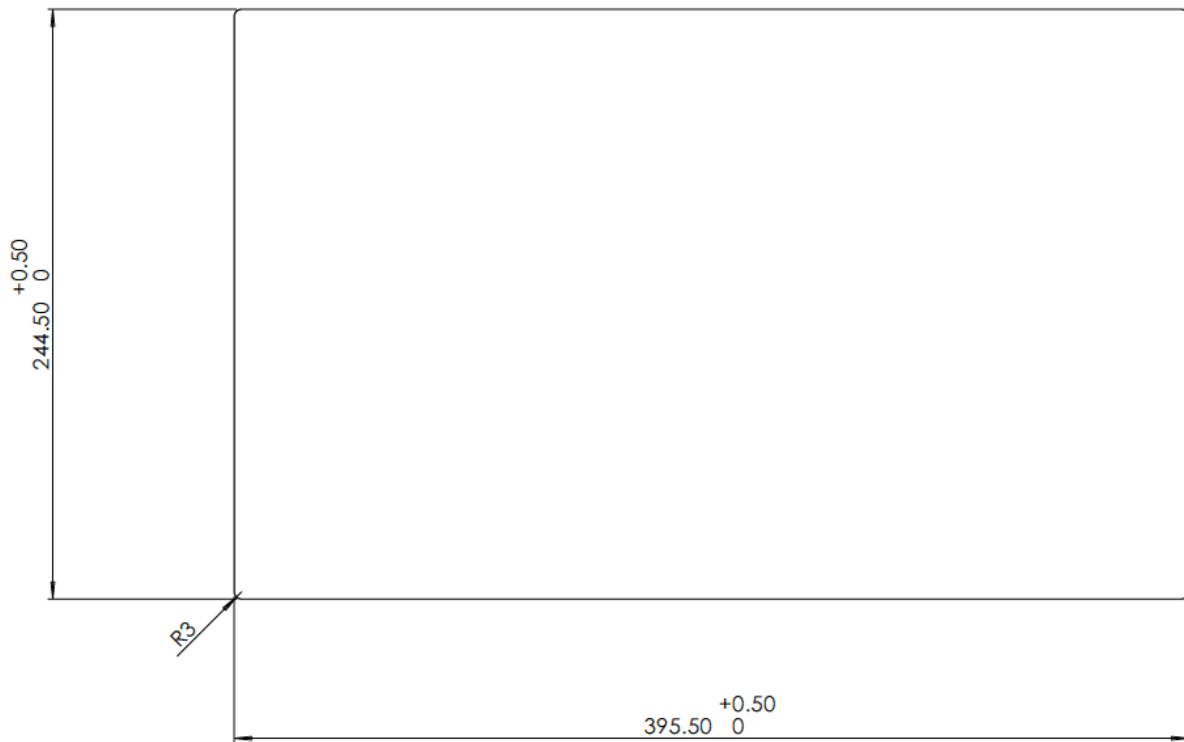
Figure 8: Mounting cut-out
