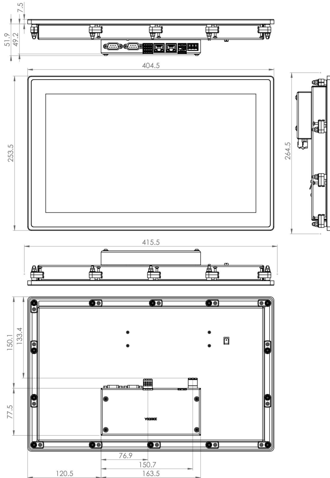
Figure 7: Dimension drawings
